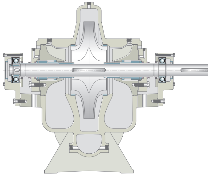
66 Bearing arrangement of a double flow pump
