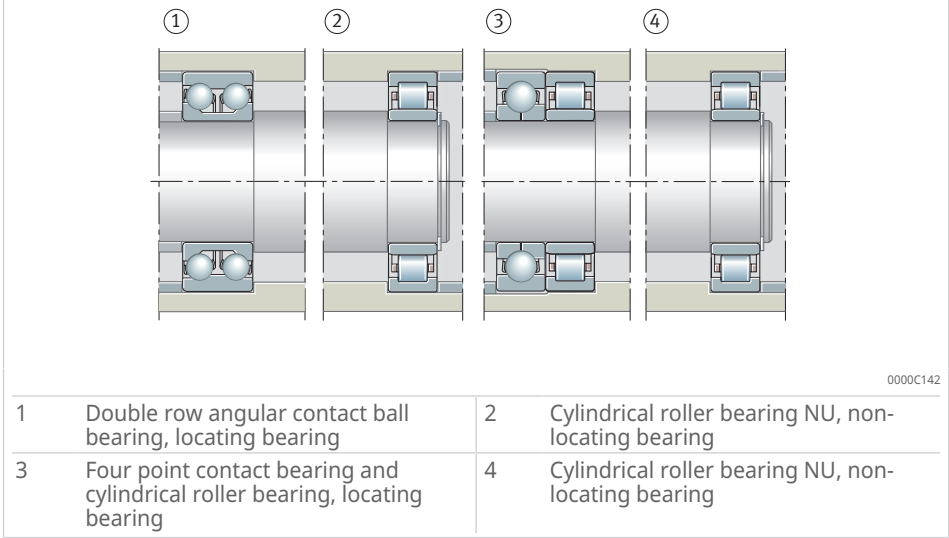
9 Locating/non-locating bearing arrangements
