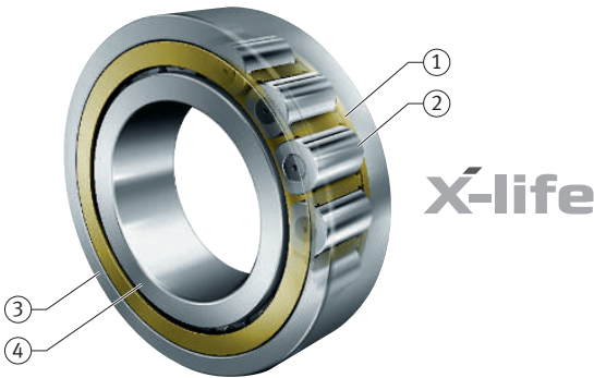
27 Single row cylindrical roller bearings in X-life design
